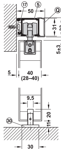
Wall mounting with mounting rail and clear threshold floor guide without guide track
