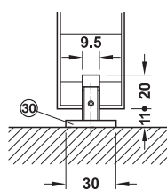
Clear threshold floor guide (30), without guide track
