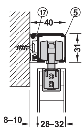
With running track (5), mounting rail (17) width 8 mm
