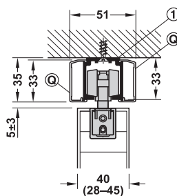
With running track (1) and 2 x clip panel (Q)
