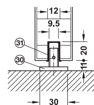
Clear threshold floor guide (30), with guide track (31)
