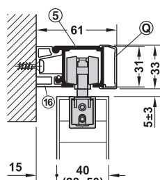
With running track (5), mounting rail (16) width 19 mm and clip panel (Q)
