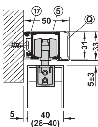
With running track (5), mounting rail (17) width 8 mm and clip panel (Q)
