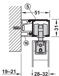
With running track (5), mounting rail (16) width 19 mm
