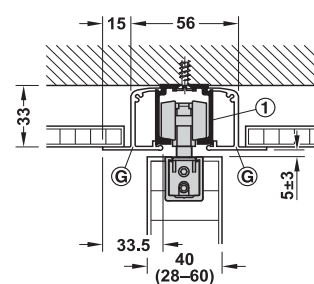
With running track (1) and 2 x clip panel (G)
